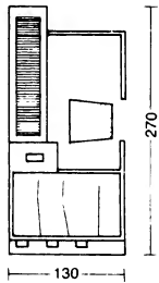
⑤ Supermarket check-out desk
